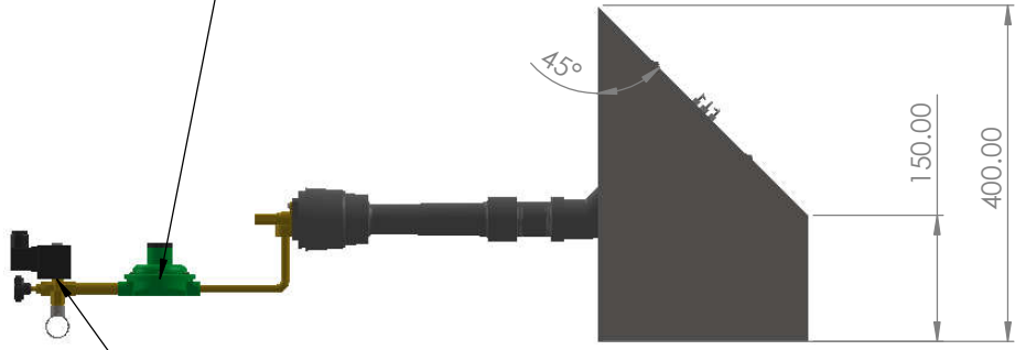
[ZCQ-01B] Flow Control Brass Solenoid Valve Gas FT-1/4", 220VAC, 0-8 bar, IP65
