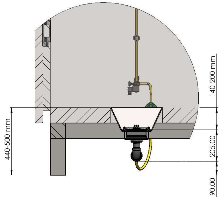
DETAIL G SCALE 1 : 10
